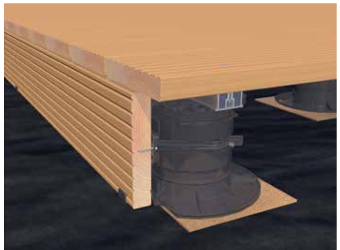
Visually appealing edging thanks to panel holder.
