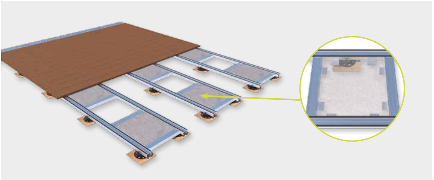
Wind suction securing in timber terraces with concrete slabs and load brackets.
