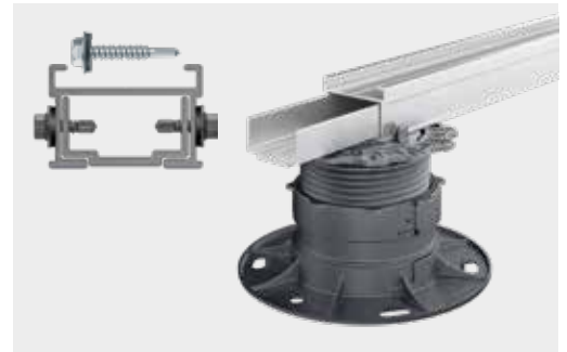
Example of fixing an EVO aluminium profile connector
