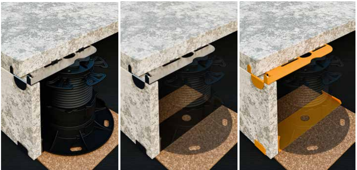
Edge finish with the PRO CERA adjustable pedestal in combination with the TERRA edge finish standalone support.
