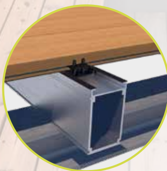
Hidden fastening using deck gliders twin system clip
