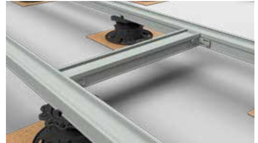
Example of application cross bracing EVO
