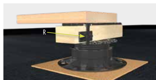
Fastening a wooden floorboard to a wooden substructure using the snap-in fastener (R).
