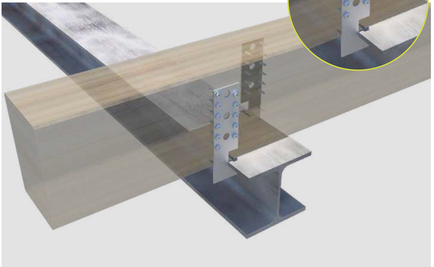
T-beam anchor in conjunction with a T-beam.
