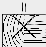
Transverse tensile reinforcement at a notch
