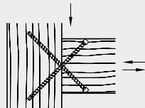
Transverse tensile reinforcement at an opening
