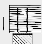
Support reinforcement
