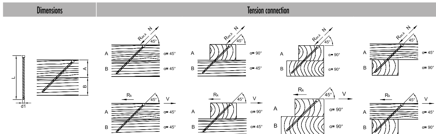
Characteristic value of the load-bearing capacity of the connection R_{ax,k} or R_k according to ETA-11/0024
